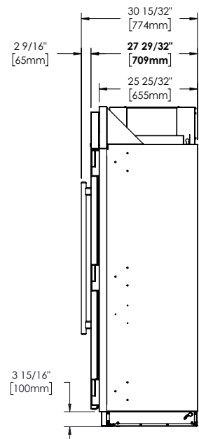
TR-36 – SIDE VIEW
