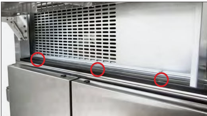
FIG. 9. Rainshield screw locations.
